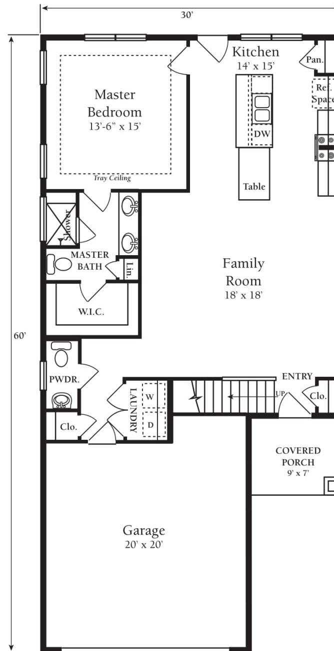
FIRST FLOOR
