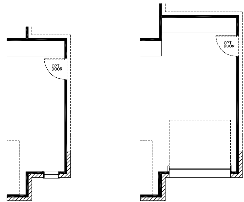
5' SIDE GARAGE EXTENSION
