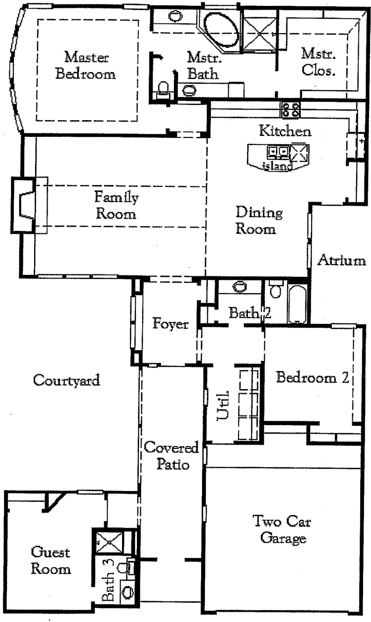
Floor Plan
