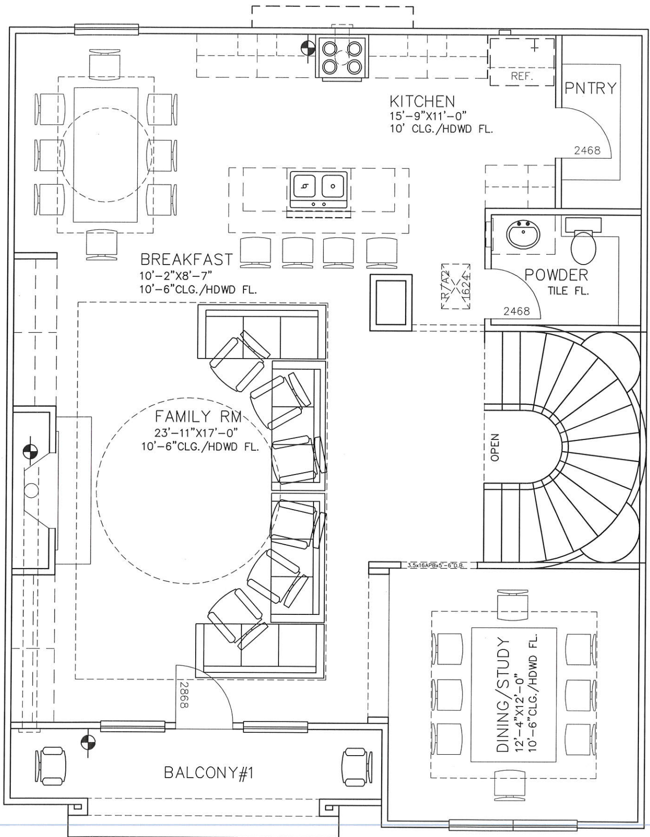
2ND FLOOR PLAN
