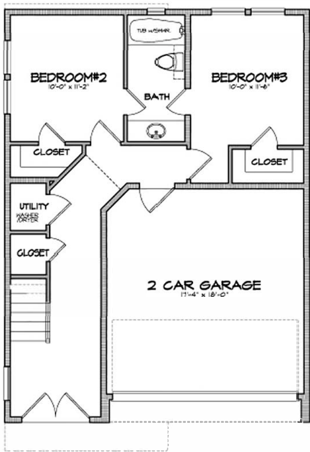
FIRST FLOOR UNIT-A
