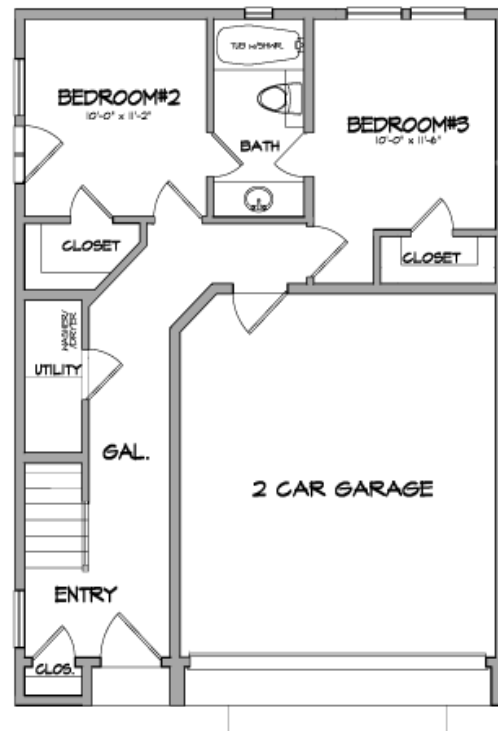
FIRST FLOOR-B
