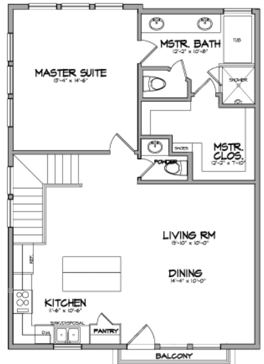
SECOND FLOOR-B
