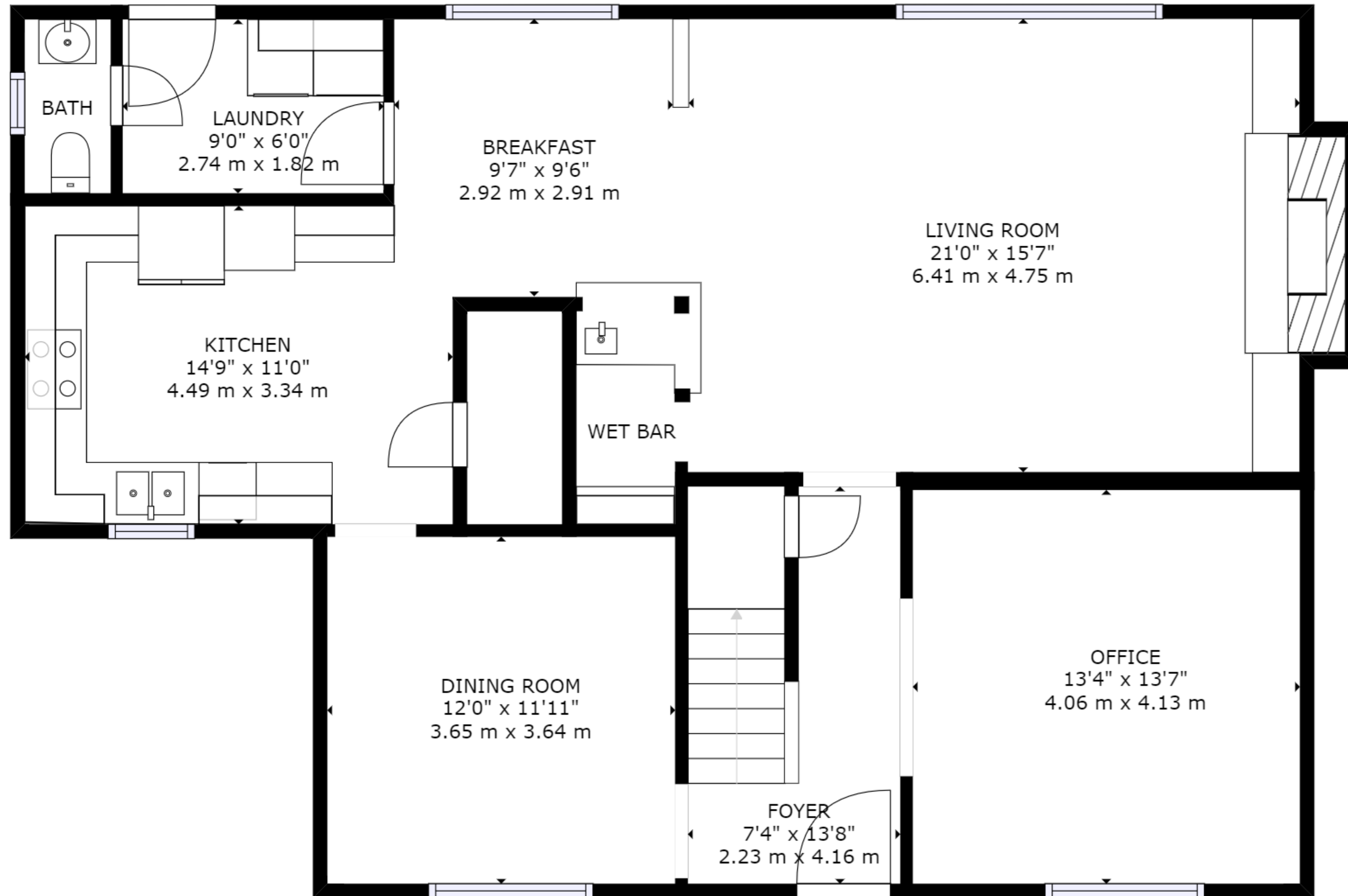
FLOOR 1
