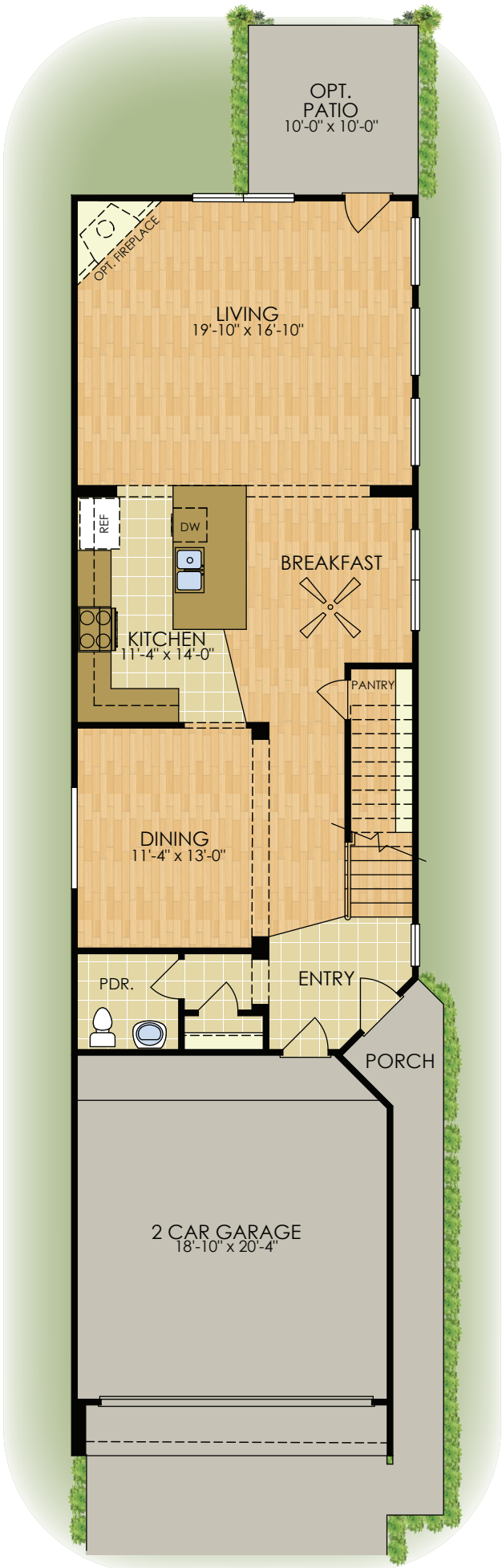
FIRST FLOOR
