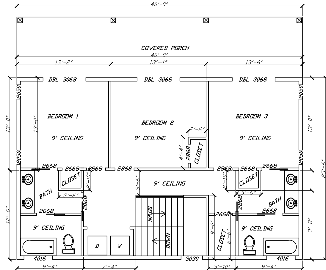
2ND FLOOR LAYOUT LIVING - 1020 FT 2 COVERED PORCH - 340 FT 2
