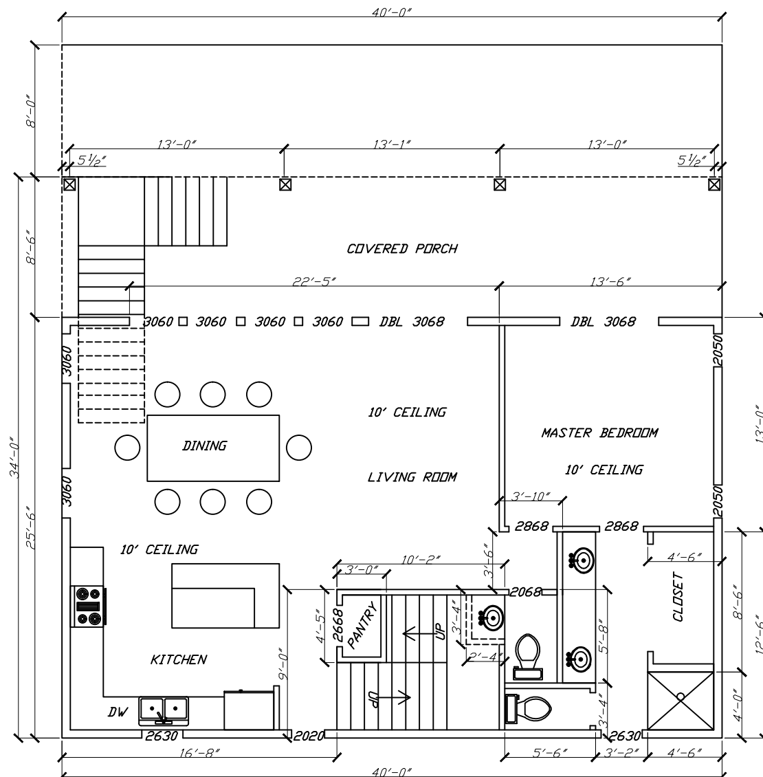
1ST FLOOR LAYOUT LIVING - 1020 FT 2 COVERED PORCH - 340 FT 2
