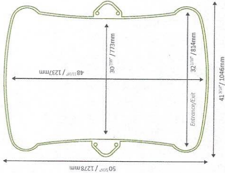
Trio Classic/Vista/Thru Weight limit: 485lb / 220kg
