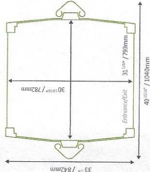
Duo Thru Weight limit: 375lb / 170kg
