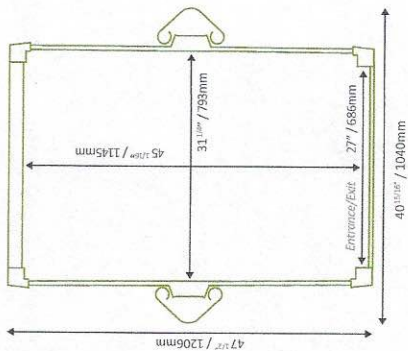
Trio Classic/Vista/Thru Weight limit: 485lb / 220kg
