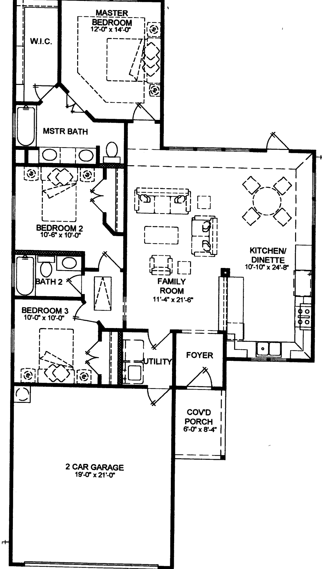
FLOOR PLAN 1321 A
