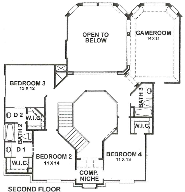
SECOND FLOOR
