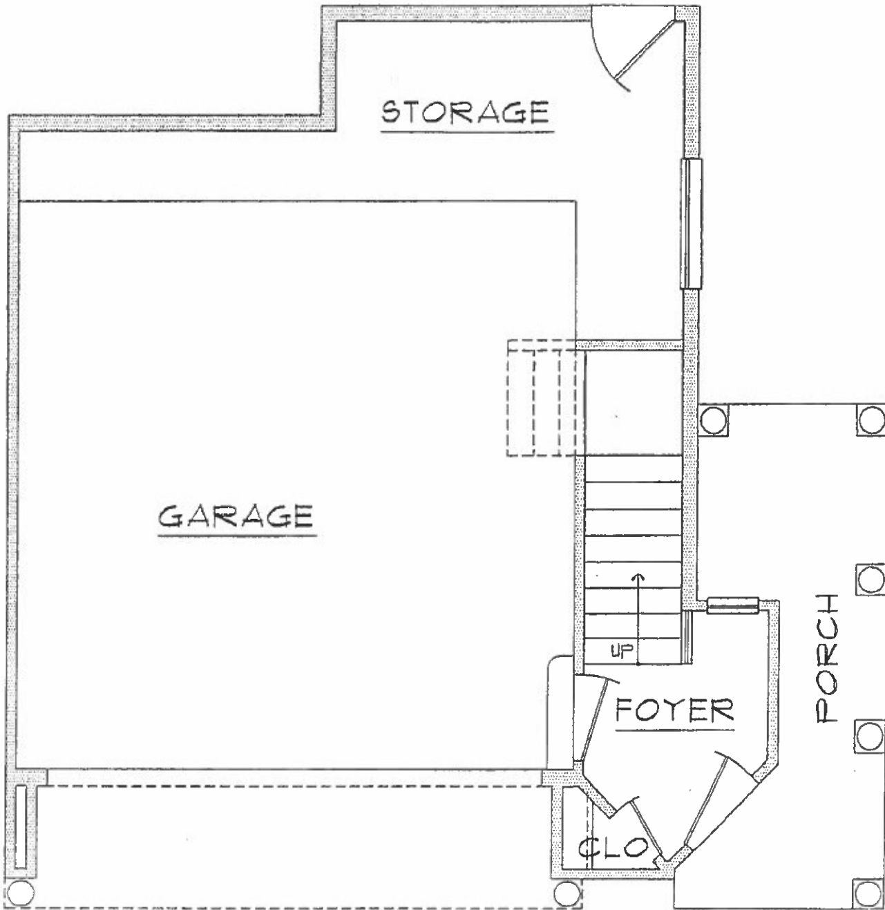
FIRST FLOOR PLAN W. 23RD
