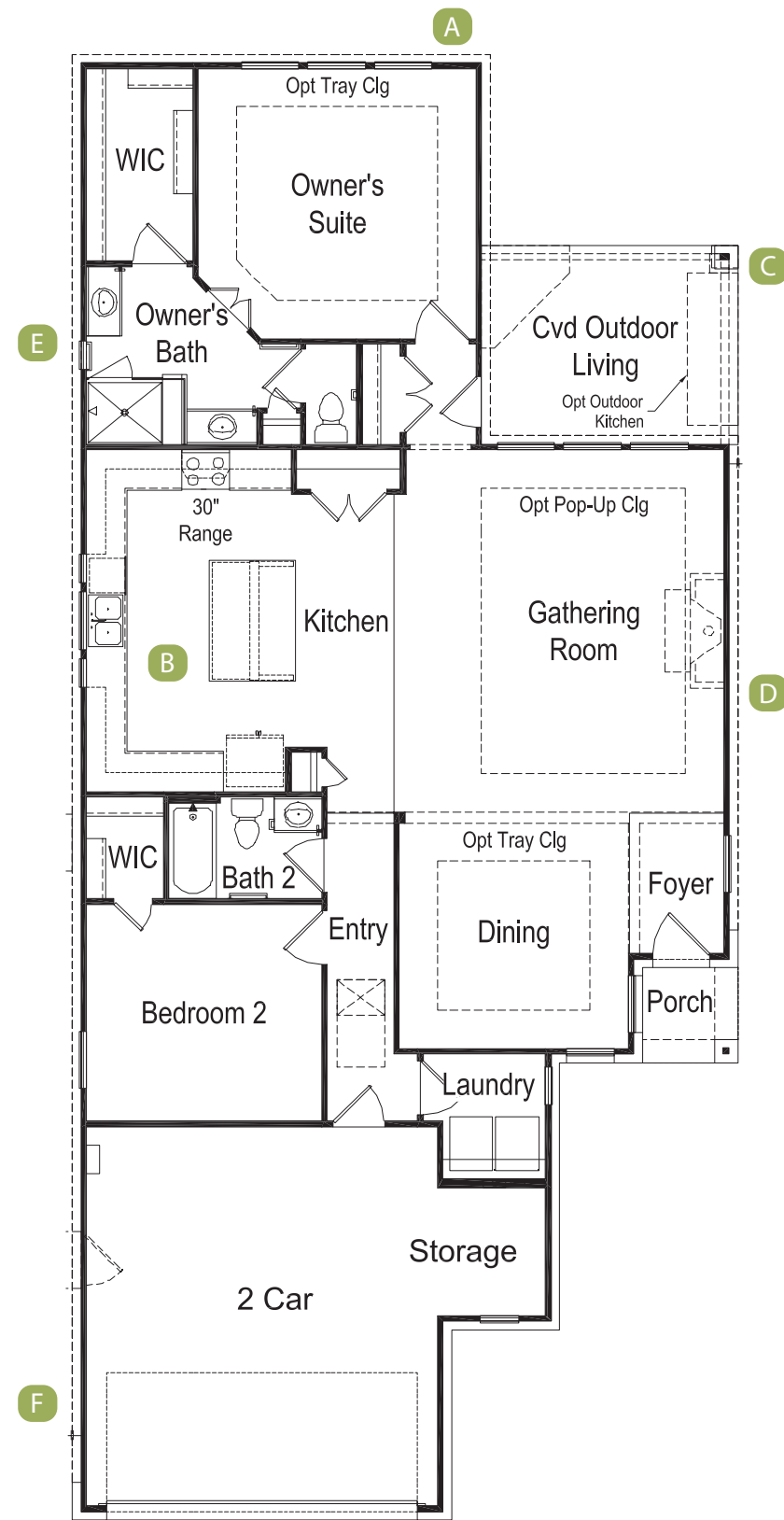
FIRST FLOOR
