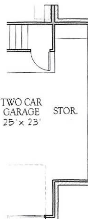
OPT. 2 1/2 CAR GARAGE
