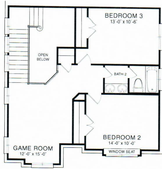
SECOND FLOOR PLAN STYLE A
