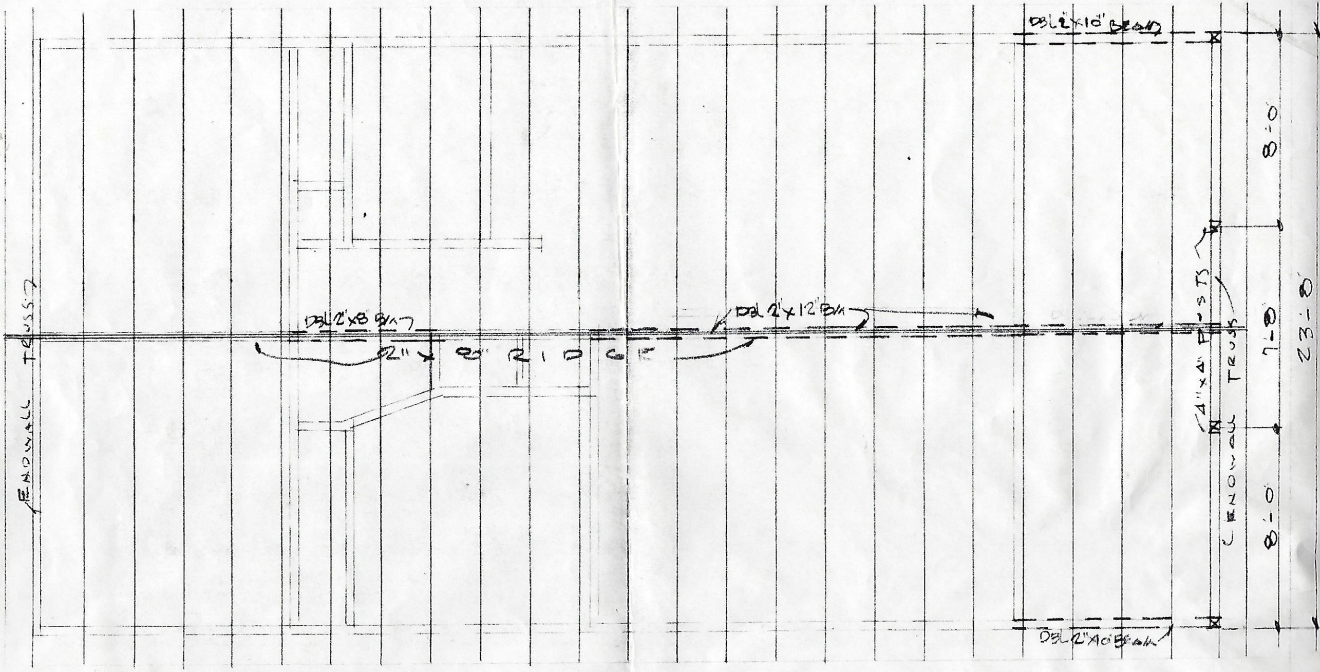
ROOF FRAMING PLAN 1/4"=1'-0"
