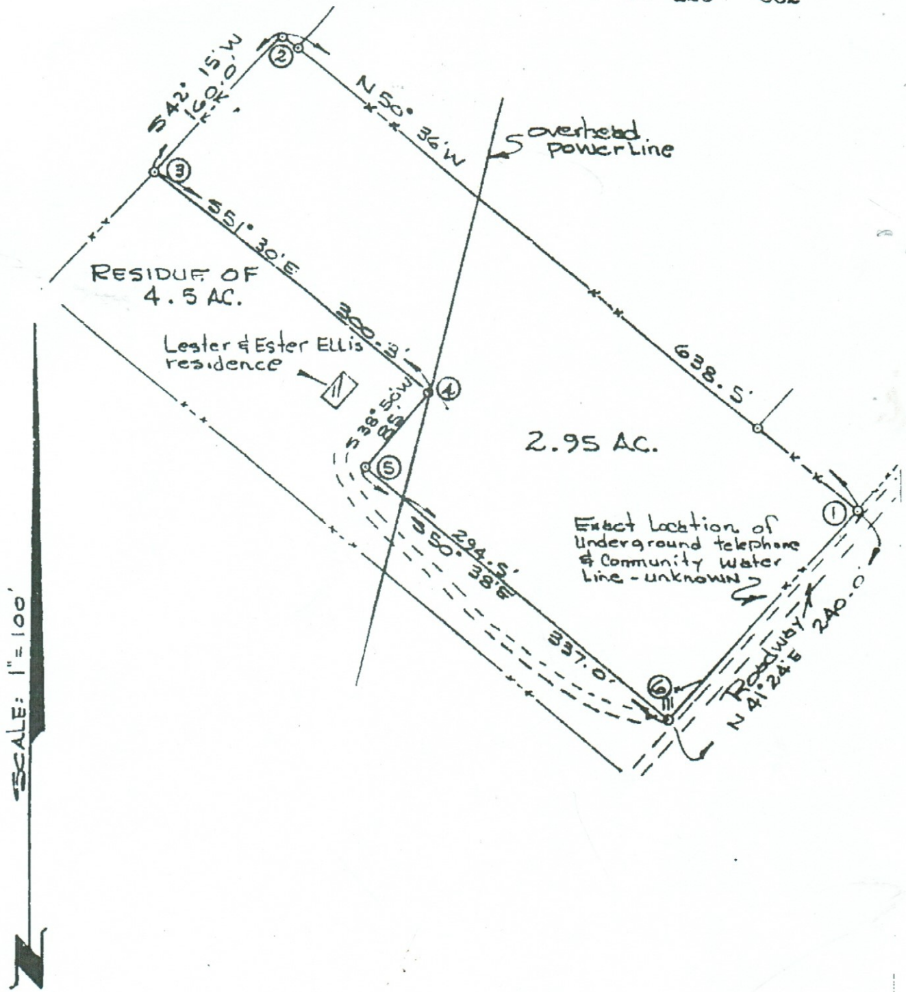
SURVEY PLAT SHOWING 2.95 AC., M/L, AS CARVED OUT OF THE LESTER & ESTER ELLIS 4.5 AC IN THE MESSINA BROWN LGE, A-5, SAN JACINTO COUNTY, TEXAS
