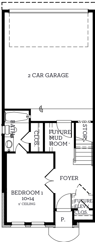
First Floor 408 sq.ft.
