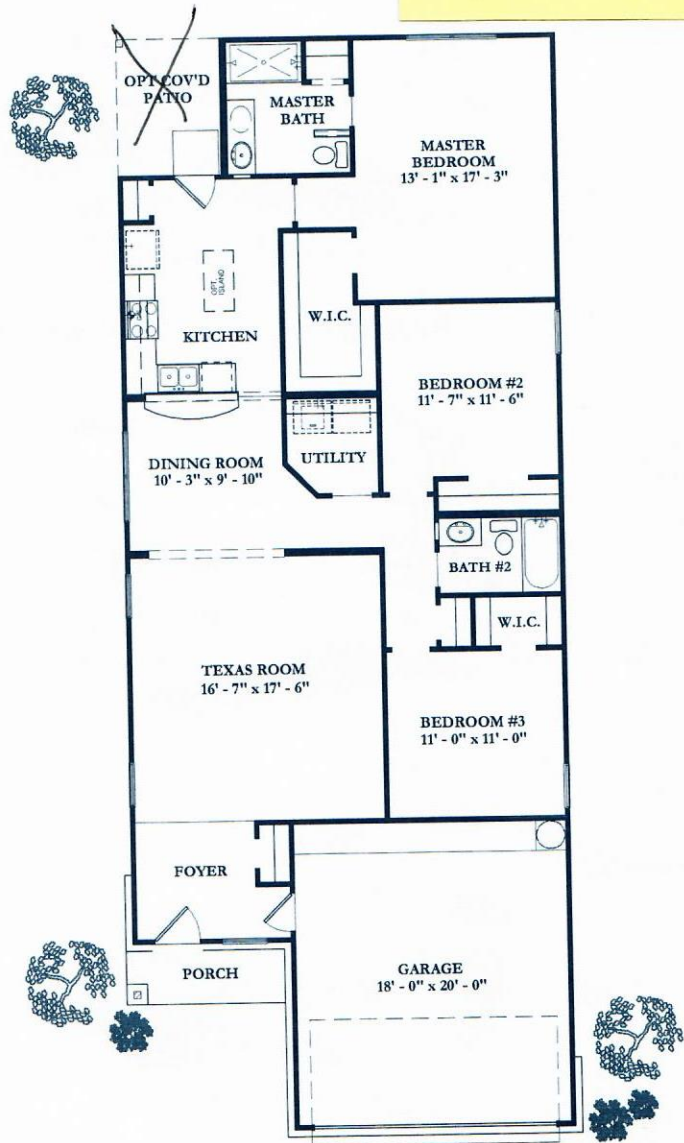
FLOOR PLAN
