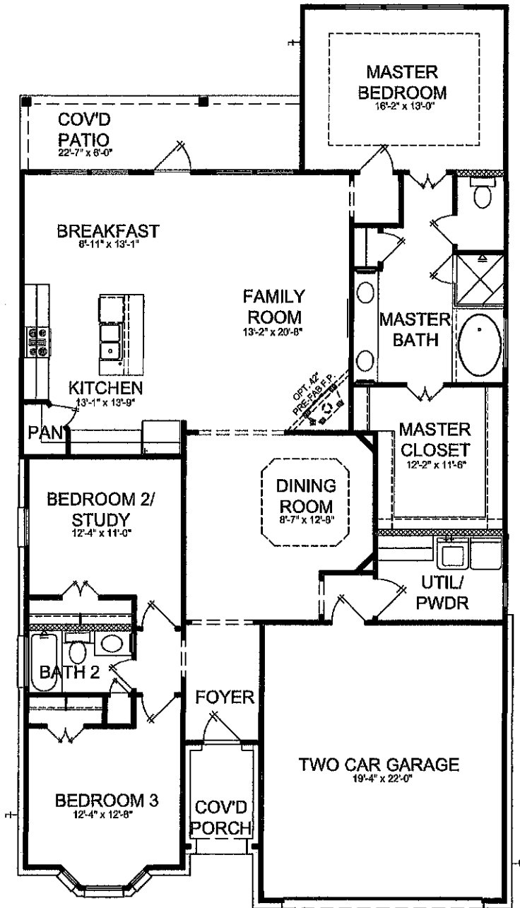
FLOOR PLAN
