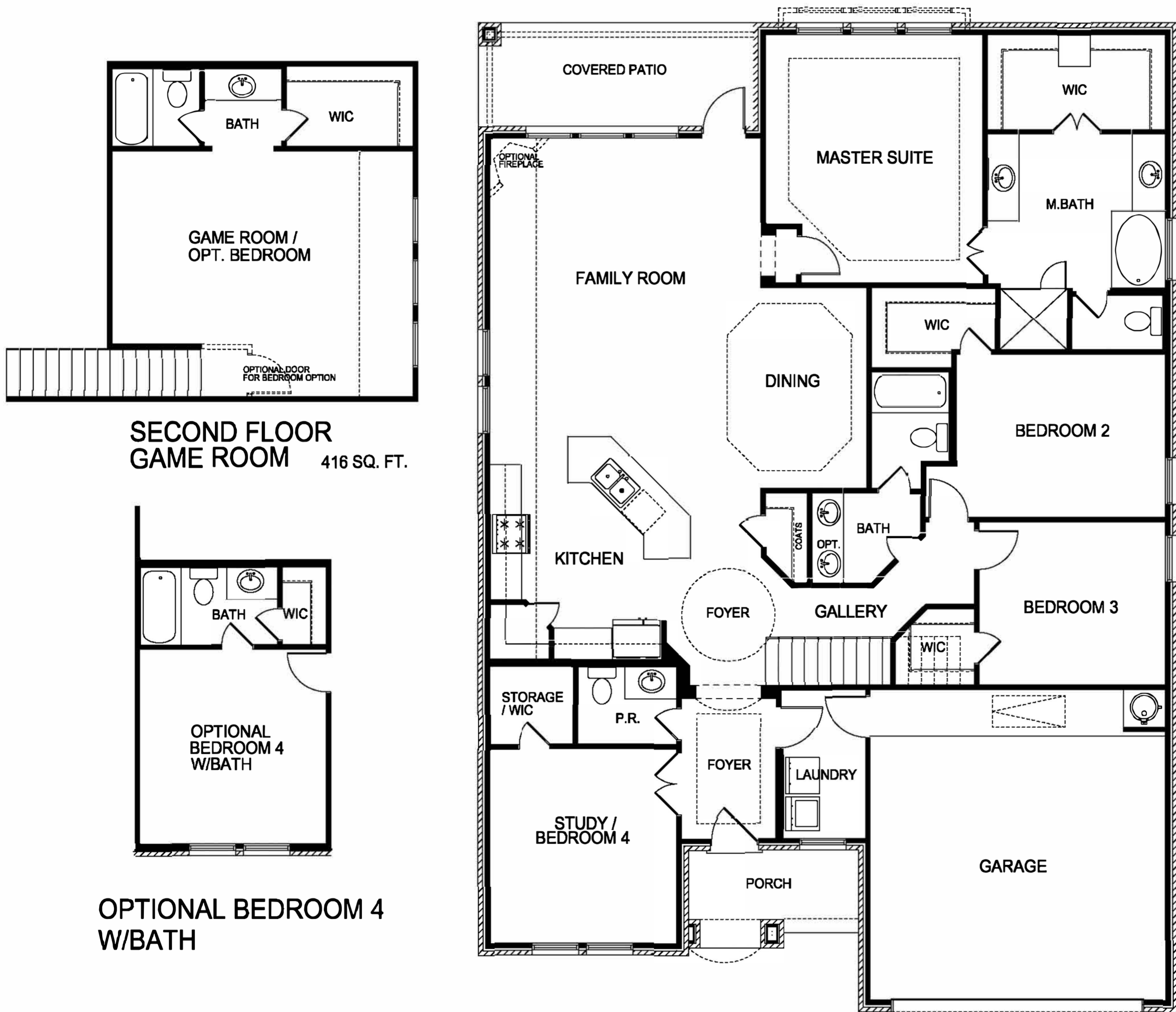
FLOOR PLAN
