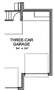
OPT. THREE-CAR GARAGE
