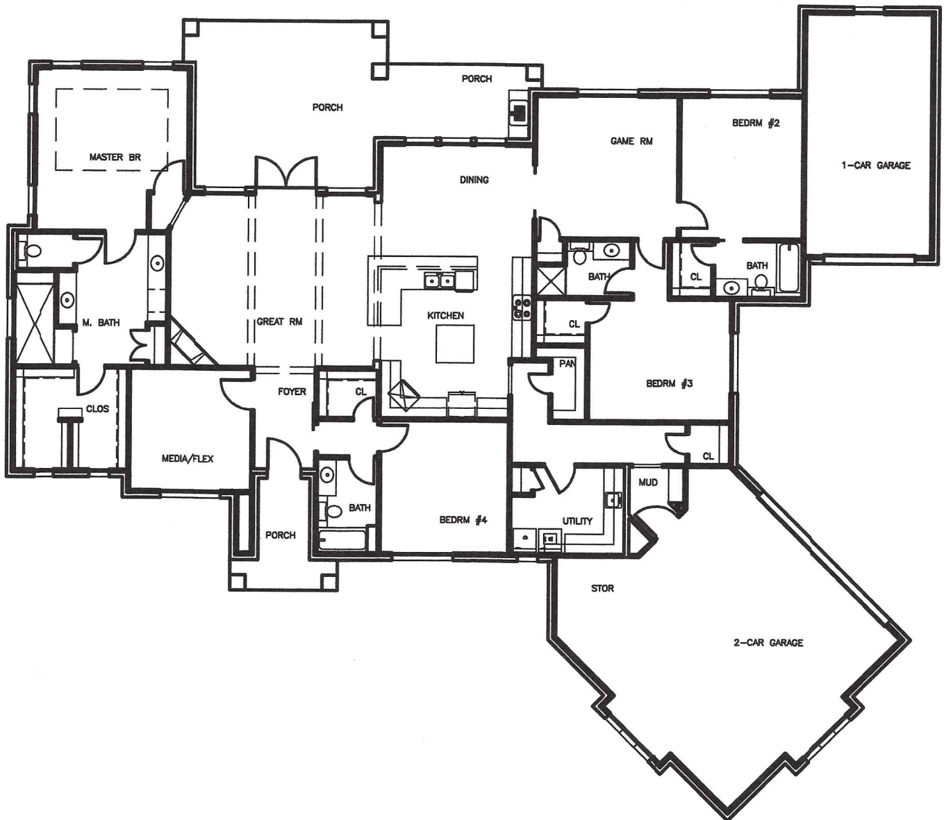
FLOOR PLAN
