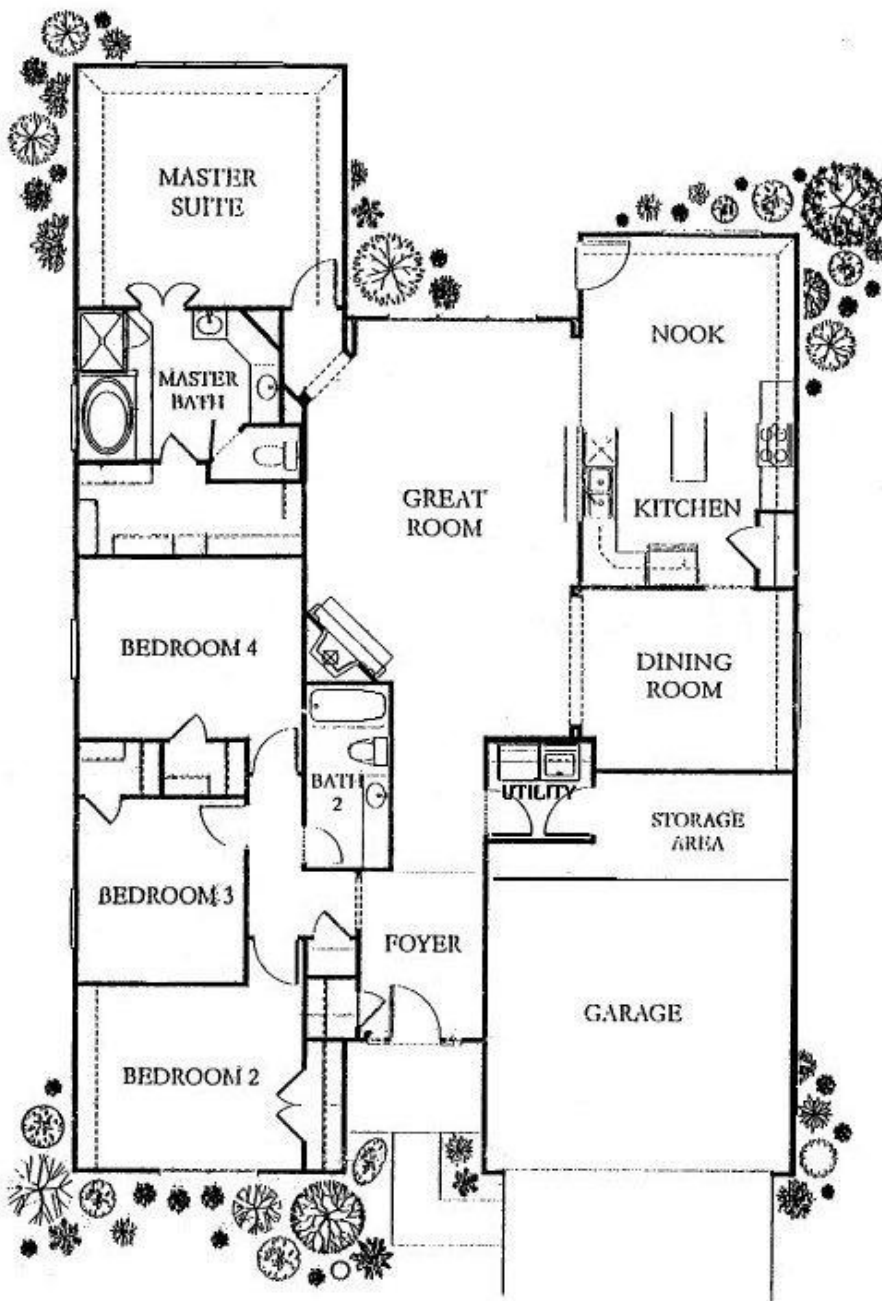
FLOOR PLAN
