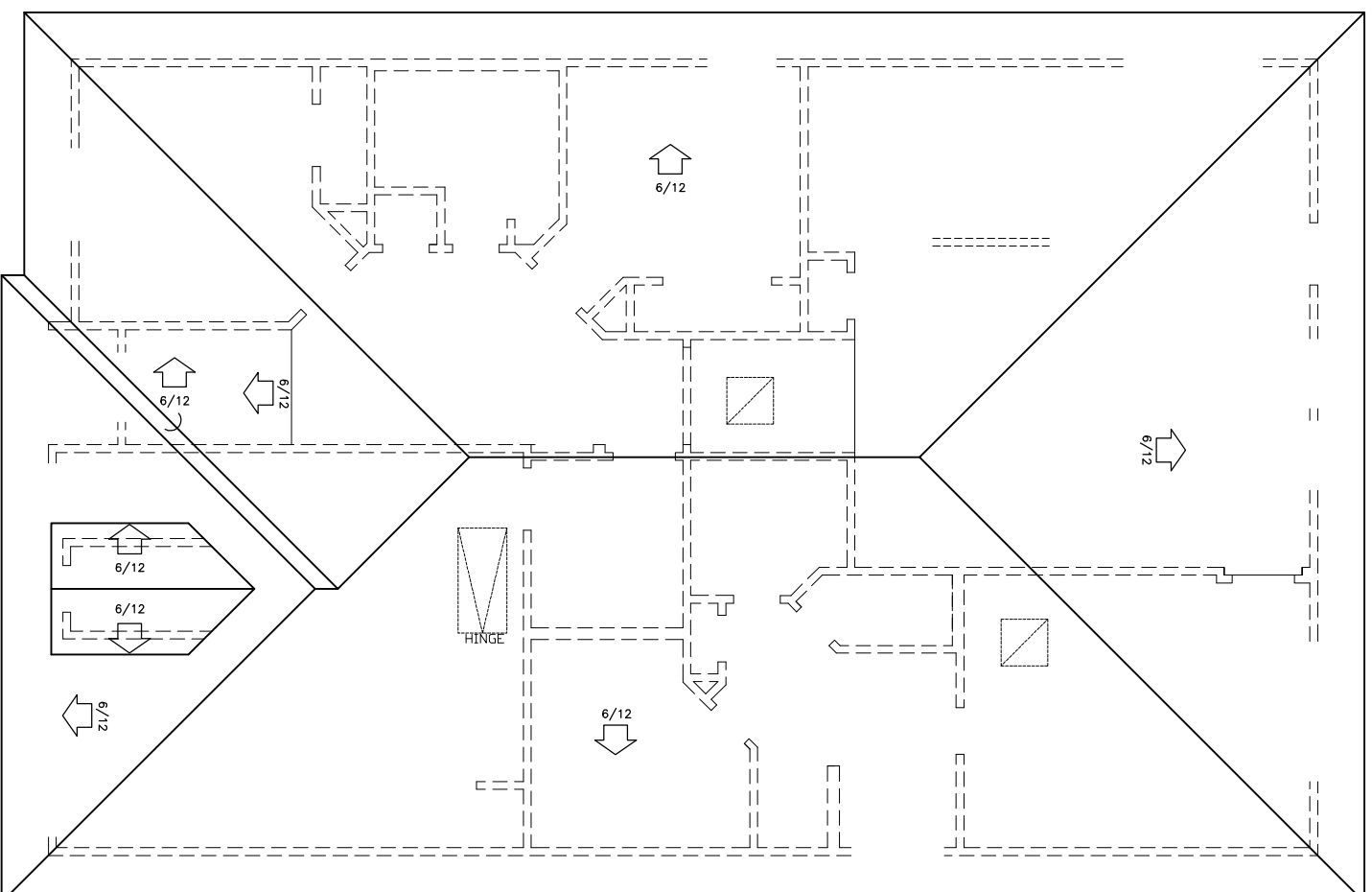
ELEVATION A ROOF PLAN NOTES: 6/12 PITCH = 1'-6" OAK (TP)
