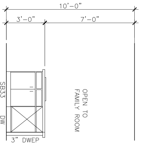
4 KITCHEN
