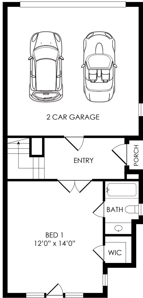
FIRST FLOOR 490 sq.ft.
