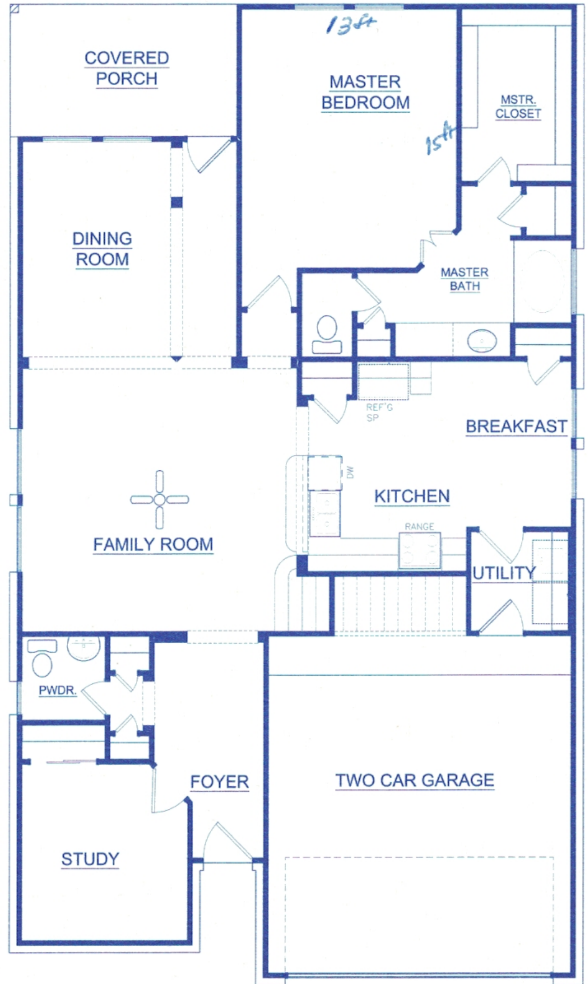
1ST FLOOR
