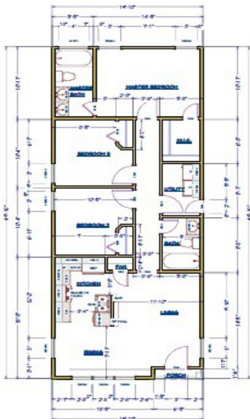
FLOOR PLAN
