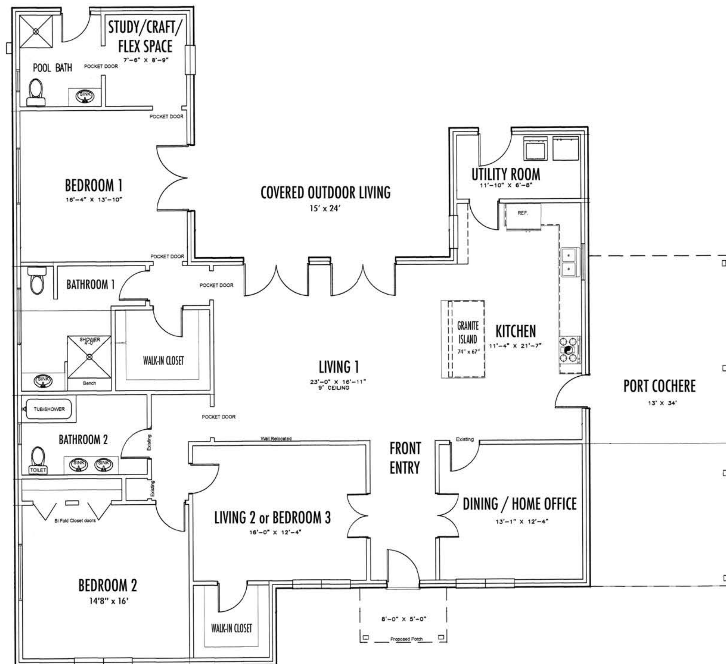
4411 O'MEARA DRIVE FLOOR PLAN
