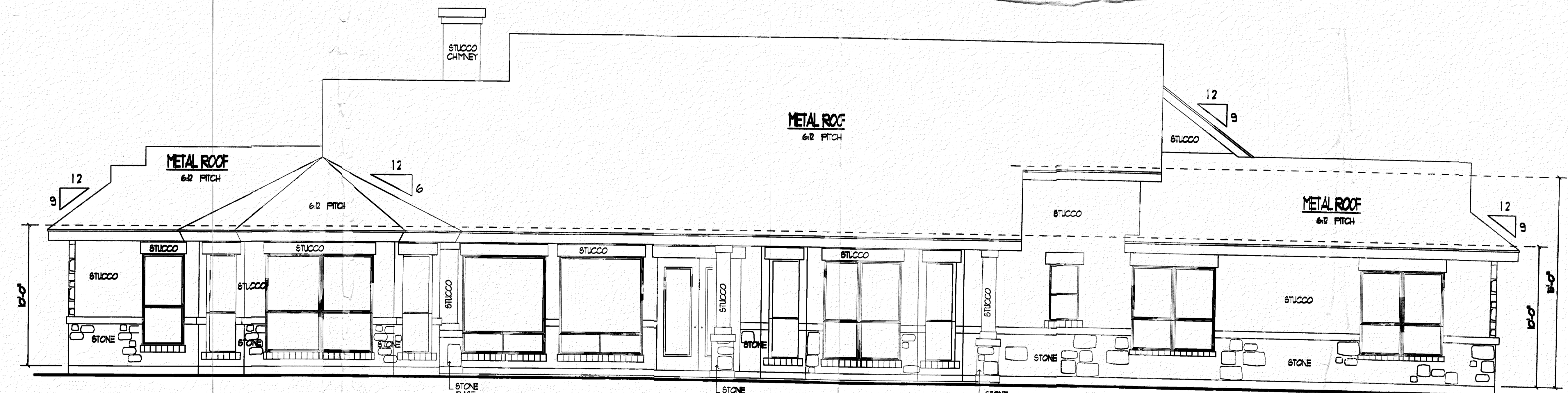
REAR ELEVATION 1/4" SCALE
