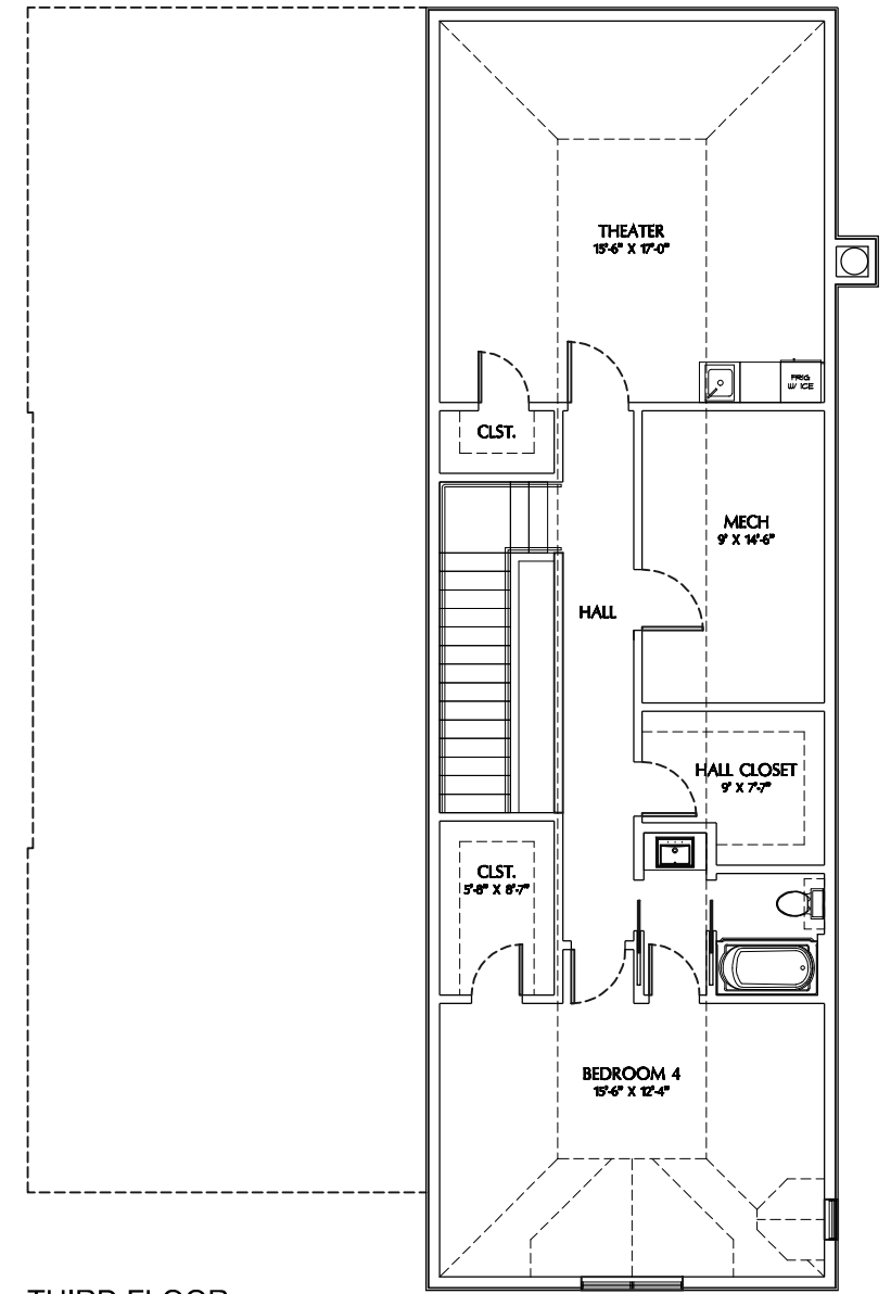
THIRD FLOOR
