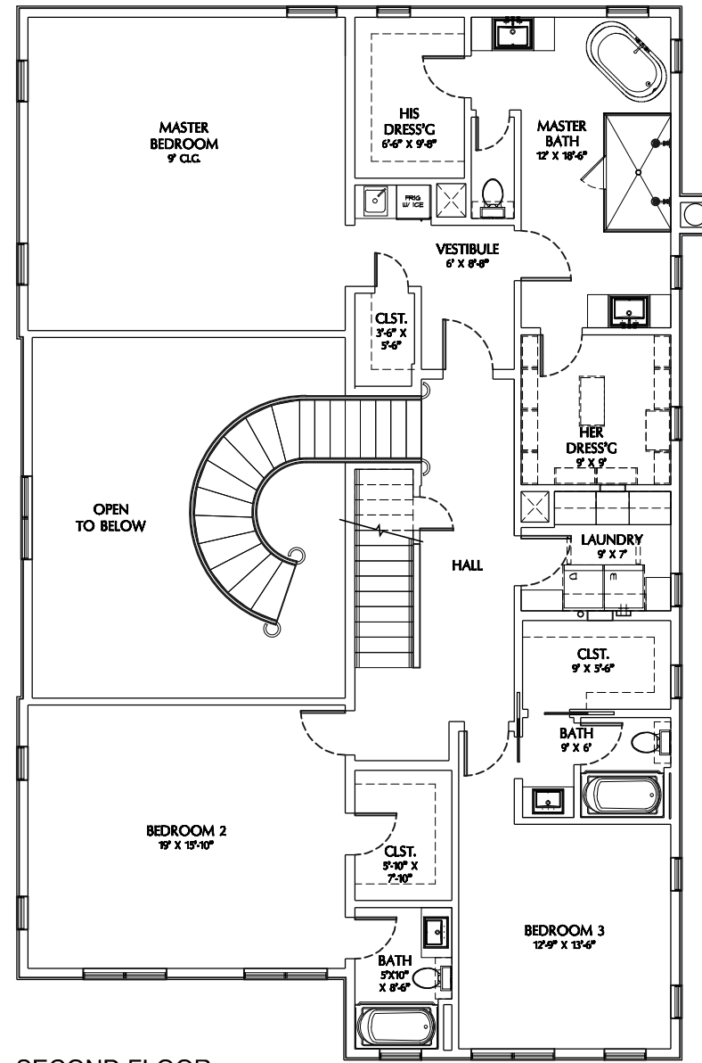
SECOND FLOOR
