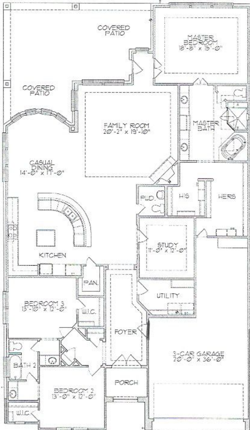
FLOOR PLAN
