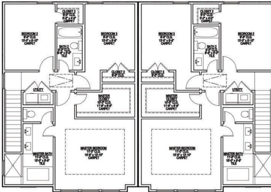
UNIT 2, 4 AND 5 2 SECOND FLOOR PLAN
