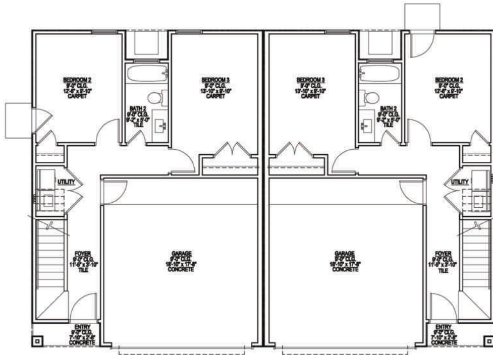
UNIT 1, 3 & 6 1 FIRST FLOOR PLAN
