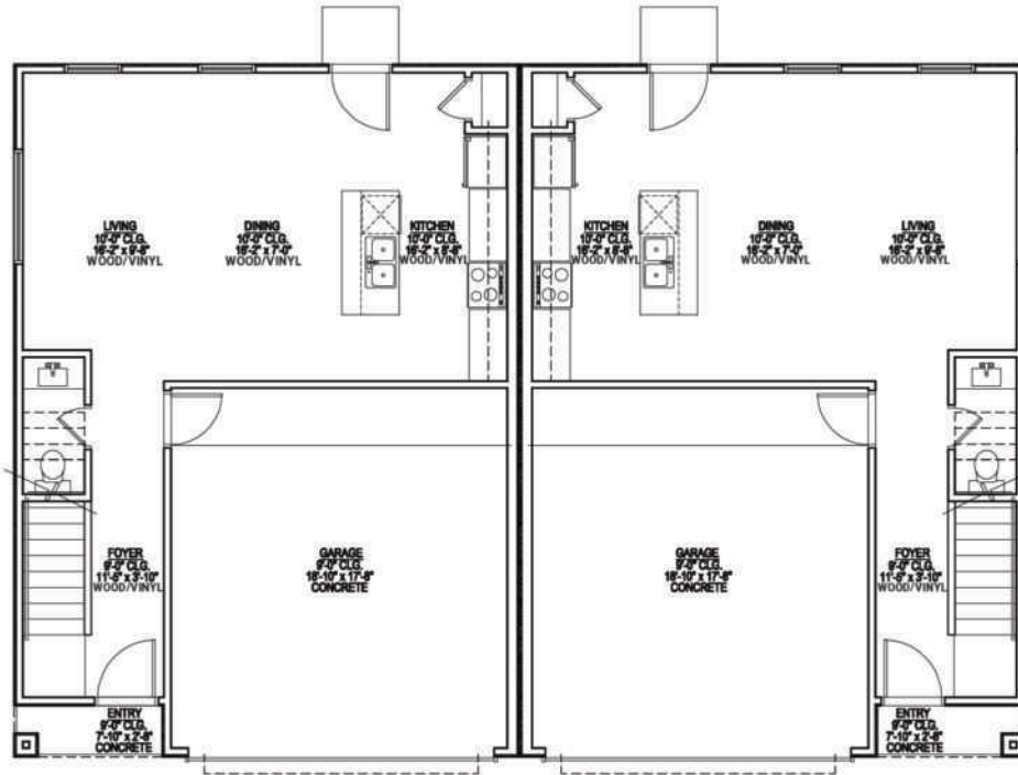
UNIT 2, 4 AND 5 1 FIRST FLOOR PLAN
