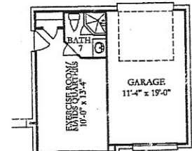
Option #0182 Maid's Qtrs./Exercise Room From 2-Car Garage +240 sq.ft.
