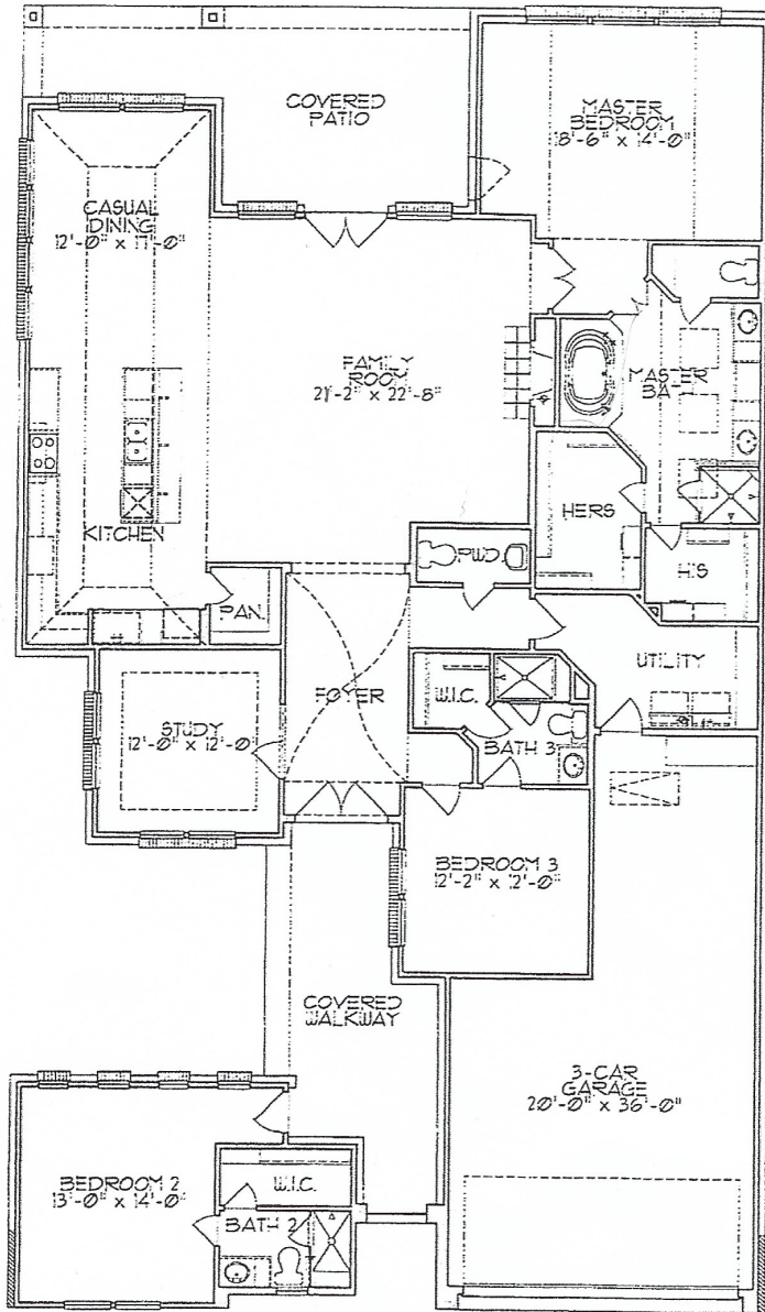
FLOOR PLAN
