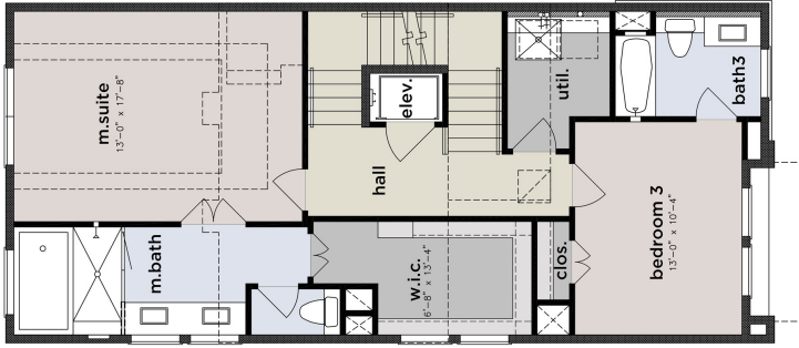
THIRD FLOOR
