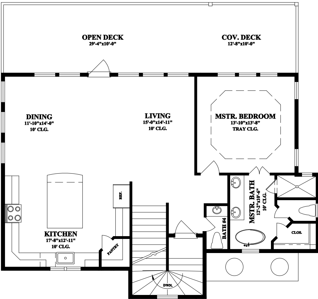
1st FLOOR LIVING 1222 Sq. Ft.
