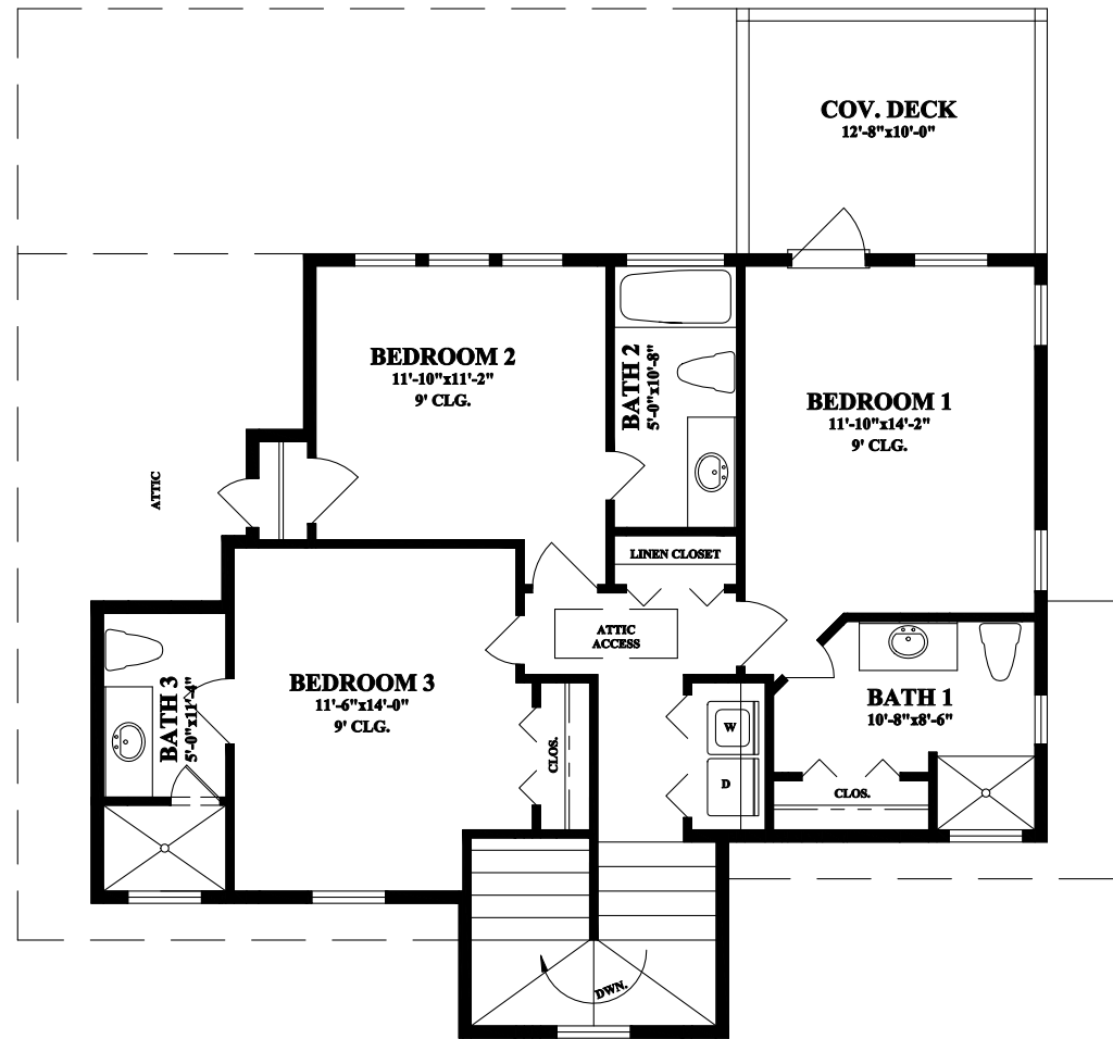
2ND FLOOR LIVING 962 Sq. Ft.
