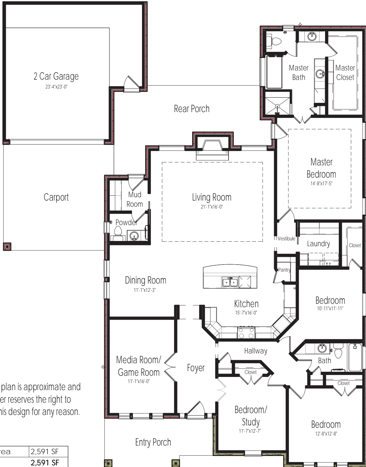
Floor Plan
