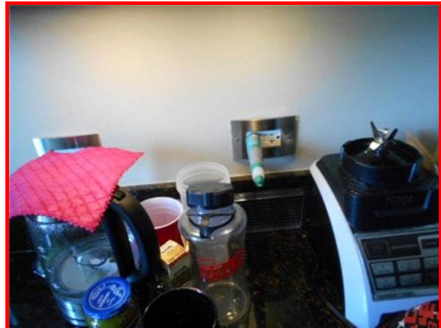
Open Neutral at Kitchen Outlet
