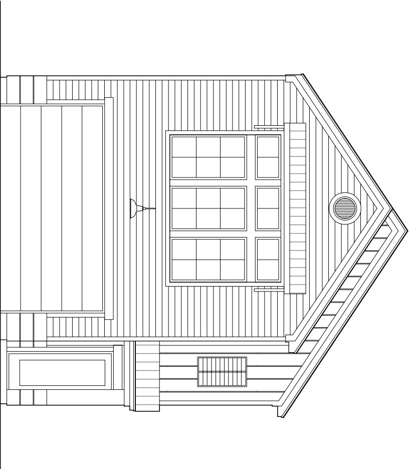
UNIT 7 ↑ FRONT ELEVATION
