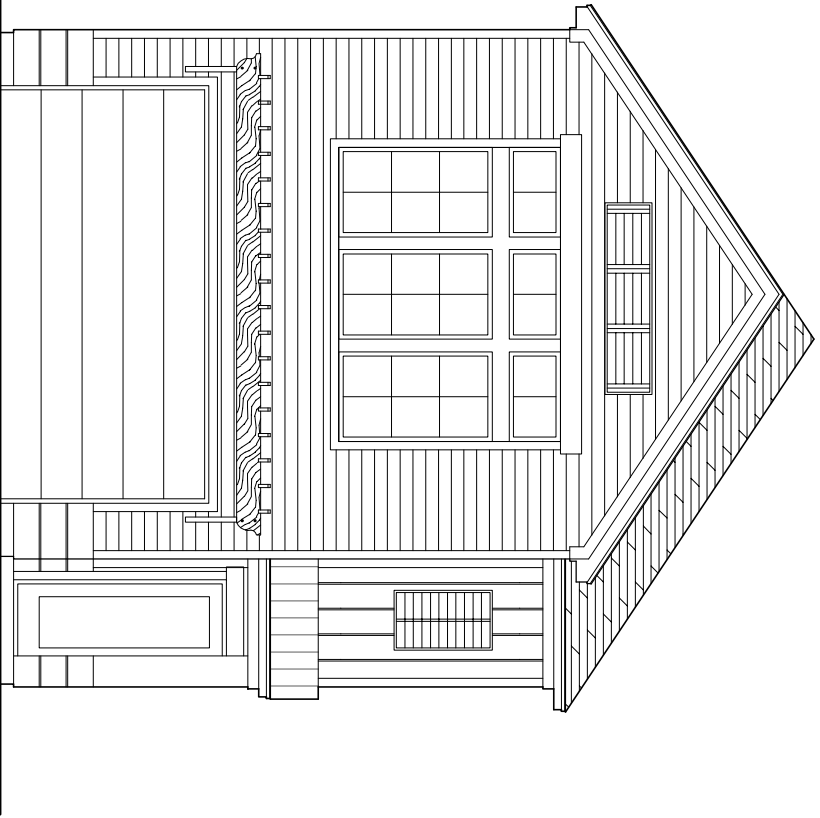
UNIT 4, 6 & 8 ↑ FRONT ELEVATION
