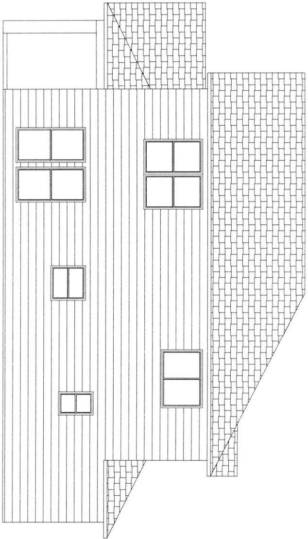
LEFT ELEVATION
