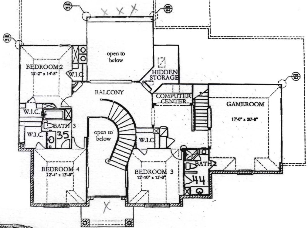
SECOND FLOOR
