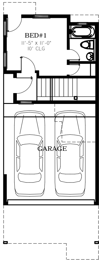
FIRST FLOOR PLAN (A)
