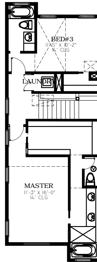
THIRD FLOOR PLAN (C)
