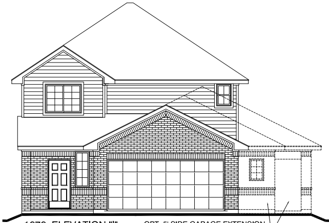
1676 ELEVATION "I" OPT. 5' SIDE GARAGE EXTENSION OPT. 3RD CAR GARAGE
