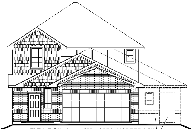
1676 ELEVATION "J" OPT. 5' SIDE GARAGE EXTENSION OPT. 3RD CAR GARAGE
