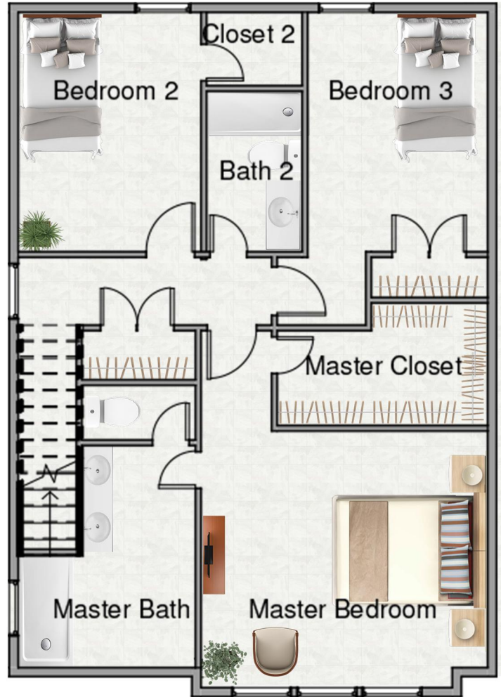
2 UNIT 2,4 AND 5 SECOND FLOOR PLAN
