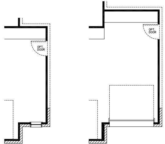
5' SIDE GARAGE OPT. 3RD CAR GARAGE EXTENSION
