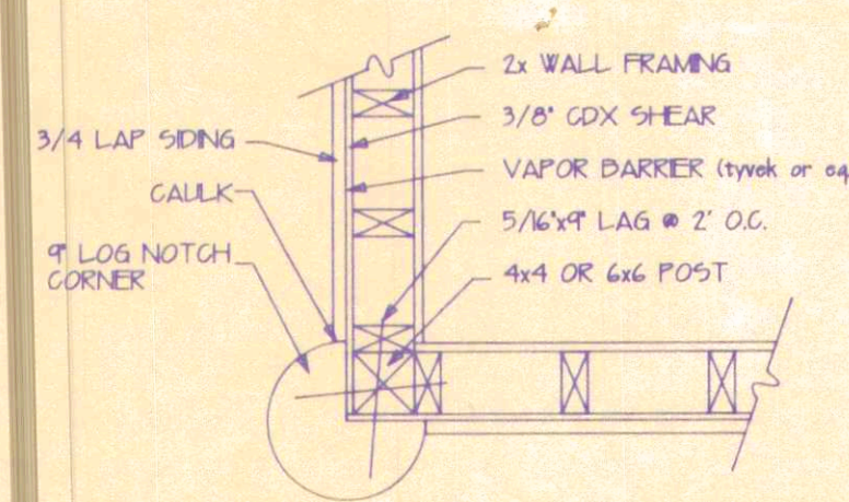
A LOG POSTS AT FRAMED WALL CORNERS
