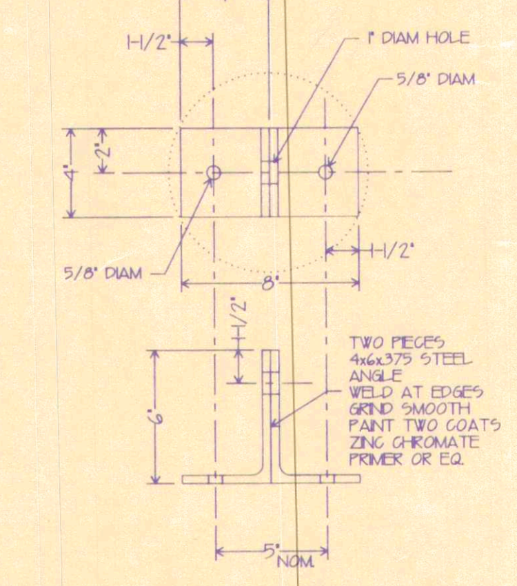
D DECK PIER T-BRACKET
