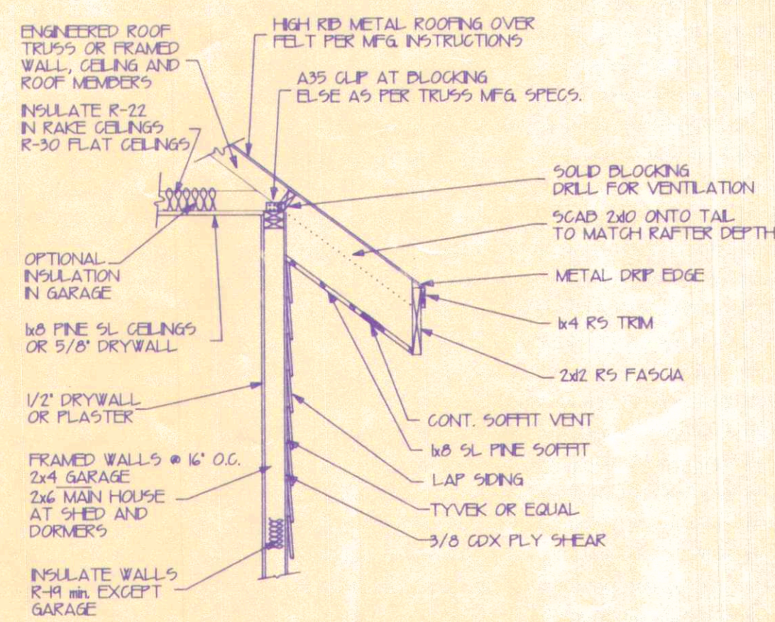
B TYPICAL FRAMED WALL AT EAVES 1/2"-0'
