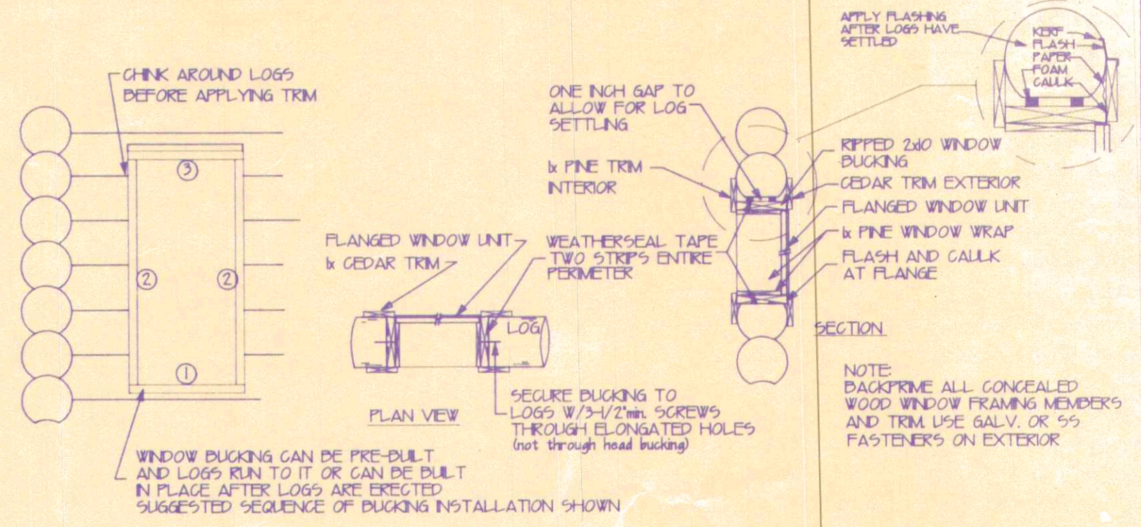
C WINDOW BUCKING AND TRIM NTS
