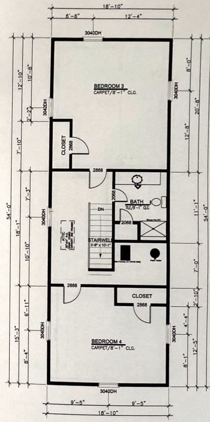
2 SECOND FLOOR 1/8" = 1'-0"
