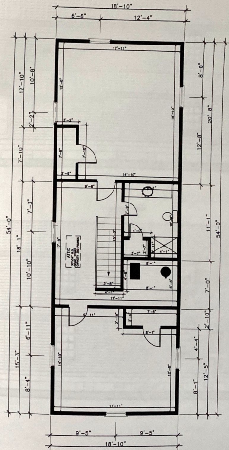
2 SECOND FLOOR 1/8" = 1'-0"
