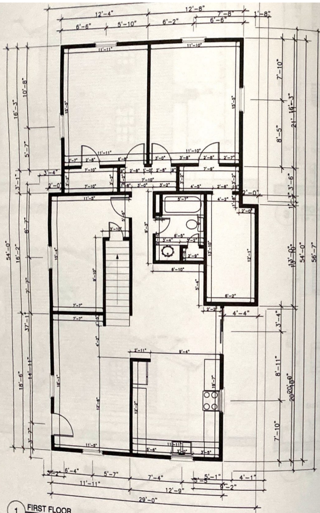
1 FIRST FLOOR 1/8" = 1'-0"
