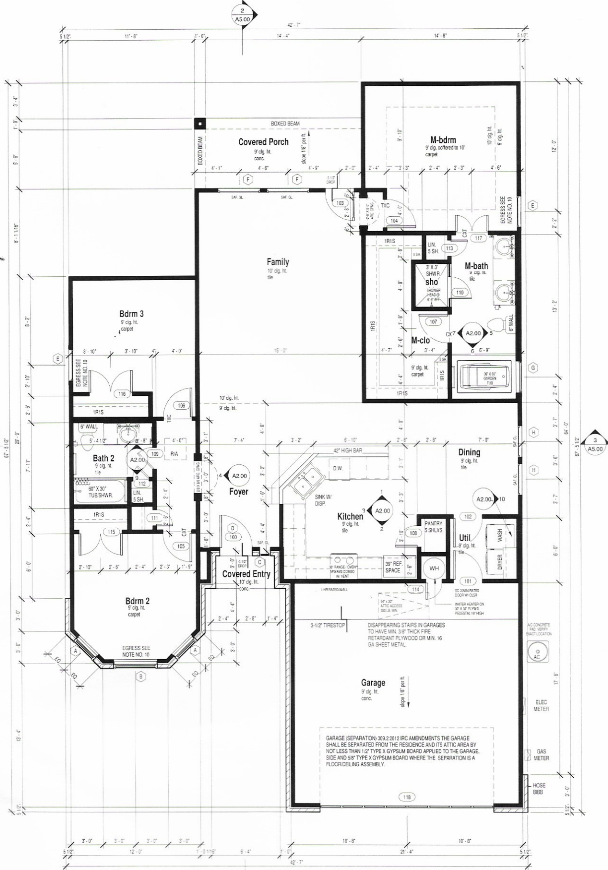
A FLOOR PLAN 1/4" = 1'-0"
